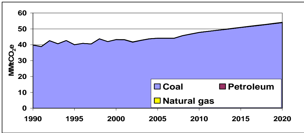
Figure A5. Wyoming GHG Emissions Associated with Electricity Production (Production-Basis)
